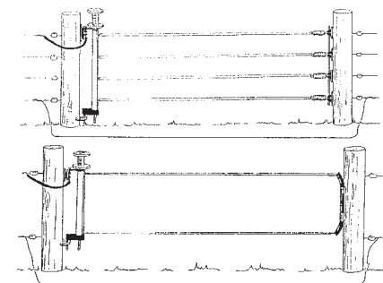
Diagram showing arrangement of 2-strand and 4-strand Taragates.
